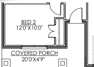
*Optional railing on porch Farmhouse elevation porch configuration
