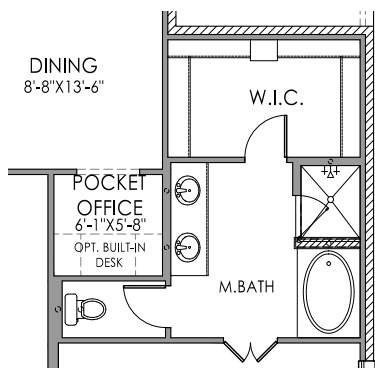
STANDARD MASTER BATH LAYOUT
