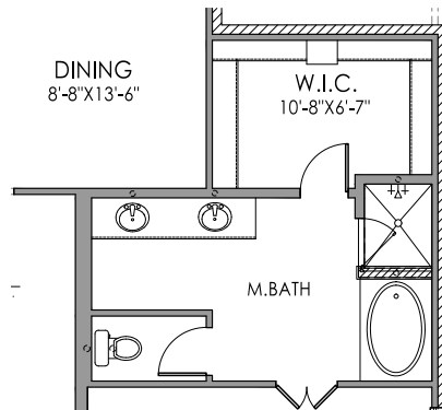
OPTIONAL LARGER MASTER BATH LAYOUT WITH LARGER VANITY (In lieu of pocket office)
