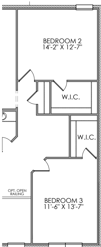
STANDARD UPPER LEVEL
