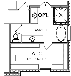
OPTIONAL MASTER BATH LAYOUT WITH SEPARATE VANITIES & LARGER W.I.C. (Adds vanity in lieu of linen closet. Reduces master bed to 14' x 17')
