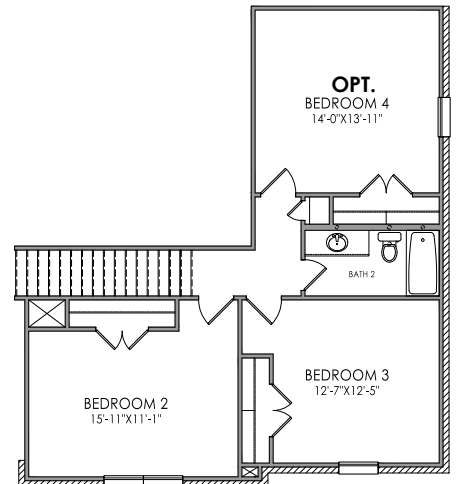
OPTIONAL BED 4 AT 2ND FLOOR Adds 275 sq. ft.
